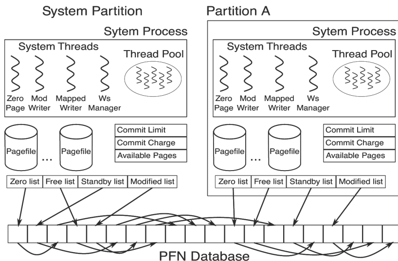
Figure 11-39. Memory partition data structures.
